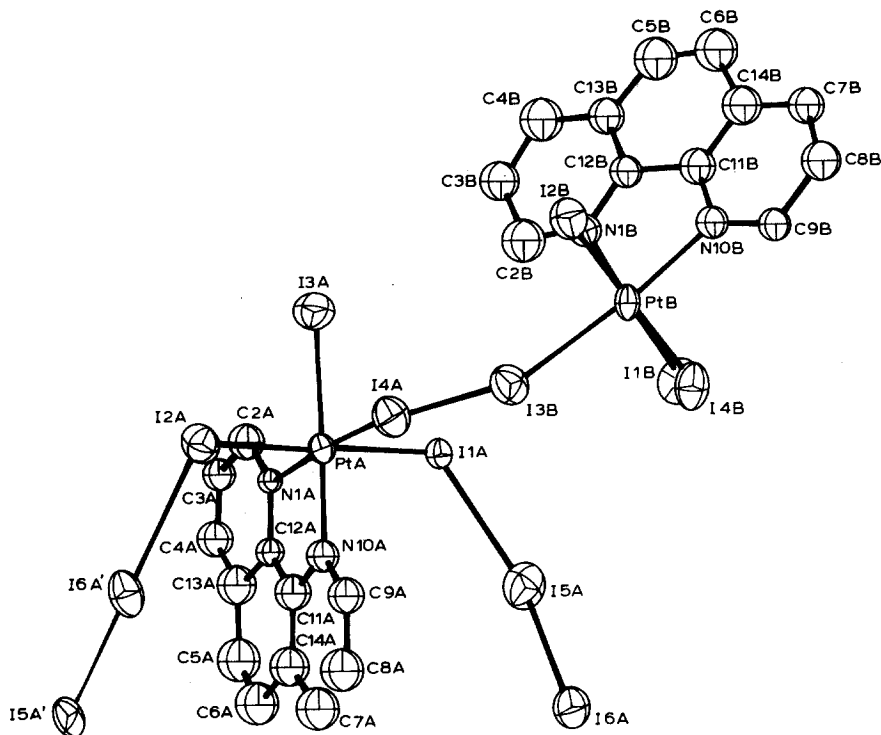
Fig. 59. The structure of [\text{Pt}(\text{phen})\text{I}_5] . From ref. 1046.
