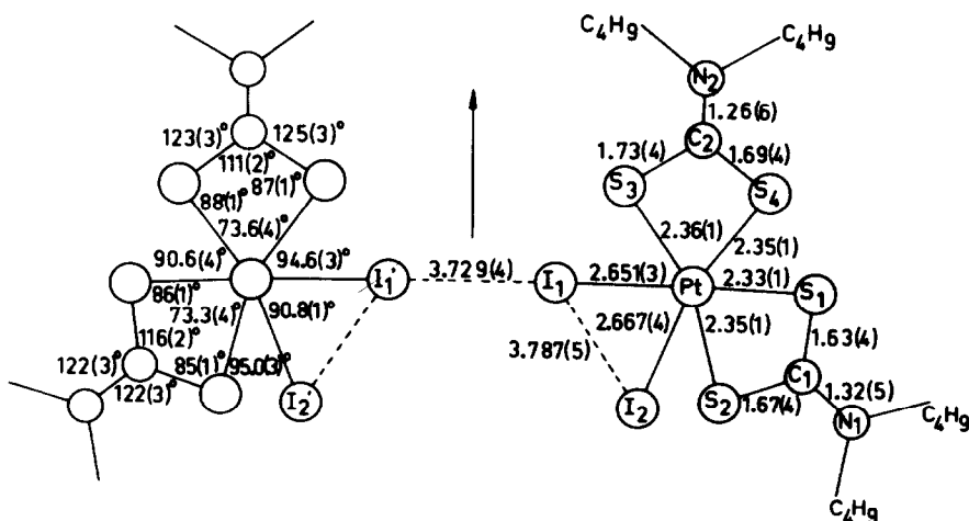
Fig. 48. The structure of \text{cis}[\text{Pt}(\text{Bu}_2\text{dtc})_2\text{I}_2] . From ref. 928.
