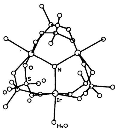
Fig. 43. Structure of the [\text{Ir}_3\text{N}(\text{SO}_4)_6(\text{H}_2\text{O})_3]^{4-} anion. From ref. 752.
