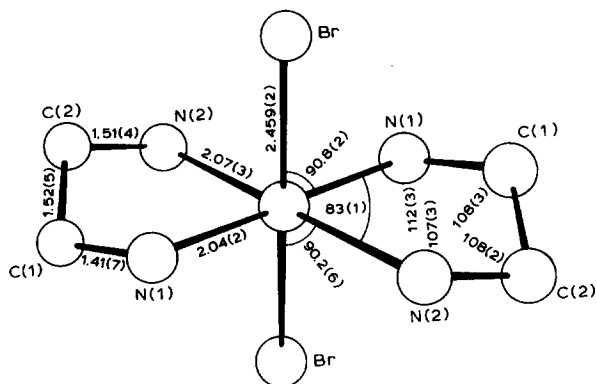
Fig. 54. The structure of \text{trans-}[\text{Pt}(\text{en})_2\text{Br}_2]^{2+} in \text{trans-}[\text{Pt}(\text{en})_2\text{Br}_2][\text{C}_4\text{O}_4] \cdot 2\text{H}_2\text{O} . From ref. 1011.
