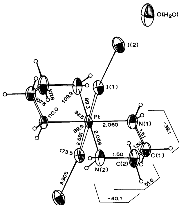
Fig. 55. The structure of \text{trans-}[\text{Pt}(\text{en})_2\text{I}_2]\text{I}_2 \cdot 2\text{H}_2\text{O} . From ref. 1012.
