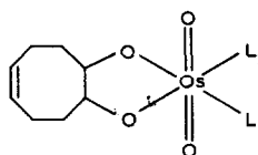
Fig. 13. The proposed structure of [\text{OsO}_2(\text{O}_2\text{R})\text{L}_2] ( \text{L}=\text{N} donor).
