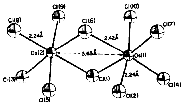
Fig. 20. The structure of \text{OsCl}_5 . Average bond angles: \text{Cl}(1)-\text{Os}(1)-\text{Cl}(6)=83^\circ ; \text{Cl}(4)-\text{Os}(1)-\text{Cl}(7)=95^\circ . From ref. 271.
