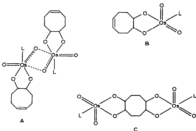
Fig. 15. The proposed structures of [\text{Os}_2\text{O}_2(\text{O}_2\text{R})\text{L}] in the solid state (A) and in solution (B) and [\text{Os}_2\text{O}_4(\text{O}_4\text{R})\text{L}_4] in solution (C).
