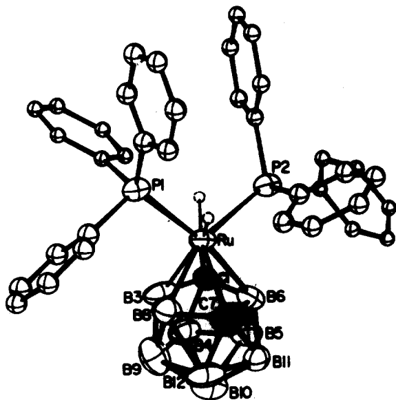
Fig. 33. The structure of [2,2\text{-(PPh}_3)_2\text{-2,2-H}_2\text{-2,1,7-RuC}_2\text{B}_9\text{H}_{11}] . Hydride atoms, which were not located, are shown as dotted circles in calculated positions. From ref. 548.
