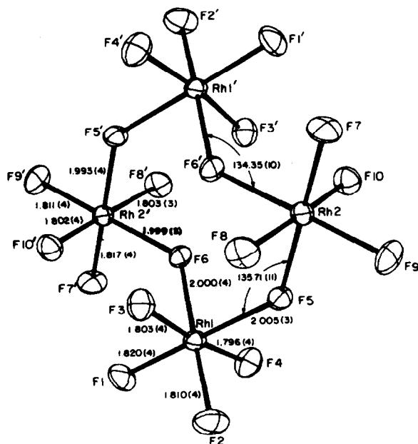
Fig. 41. Structure of the \text{RhF}_5 tetramer. From ref. 613.
